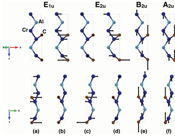
Figure 3. Schematic representation of the atomic displacements for the six highest phonon energy modes at \Gamma . (a,c) in-plane transverse optical modes, (b,d) in-plane longitudinal optical modes and (e,f) out-of-plane transverse optical modes. The arrows (eigendisplacement \times atomic mass) schematically represent the atomic displacement for the specific vibration mode.
