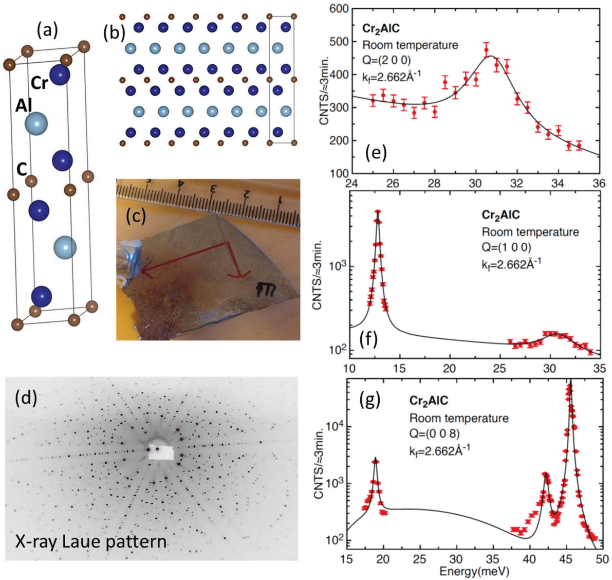
Figure 1. (a) and (b) atomic structure of Cr 2 AlC (P6 3 /mmc space group, a = 0.286 nm, c = 1.282 nm) (c) Photograph picture of a Cr 2 AlC single crystal used for measurements. (d) Transmission Laue diffraction pattern (the longer red axis in (c) corresponds to the horizontal direction in (d)). Crystal shape corresponds to a vertical cross section of the crucible shape and solution surface, which ultimately limit crystal expansion. (e), (f) and (g) are selected inelastic neutron scattering phonon spectra measured for scattering vector values indicated in the Figure. Lines are fits of the data with harmonic oscillator line shape. The scattering vector Q is decomposed into Q = G + q , where G is a reciprocal lattice wavevector and q is the wavevector of the excitation.
