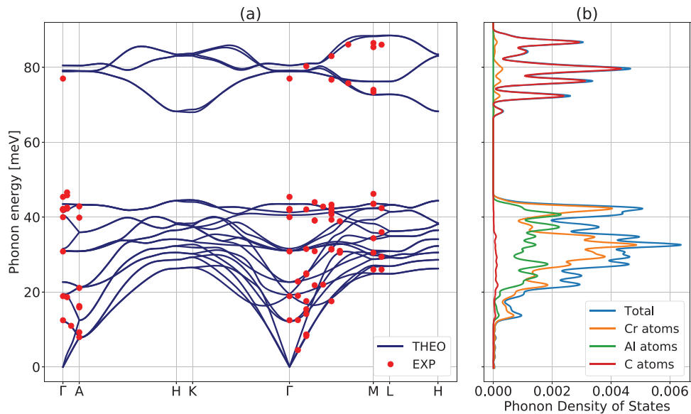
Figure 2. (a) First-principles phonon spectrum and experimental phonon energy modes of Cr 2 AlC along major crystallographic directions and (b) corresponding theoretical phonon density of states separated among the various atomic constituents.
